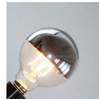
toshi LED Globe Filament (65mm) 0501 Kopfspiegel / top mirror globe / globo con cupula espejada Ø 95 mm, 4W, 450LM, 2700K, EEK: A++
